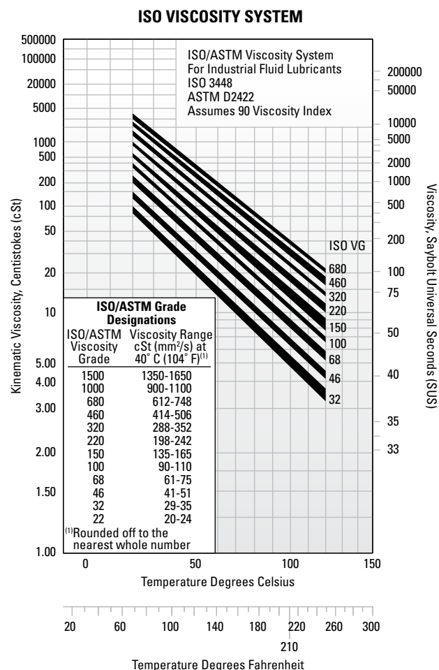
Fig. 20. Viscosity grade system for industrial oils.
