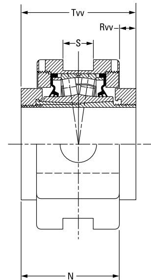
QVV Double-Nut Unit
