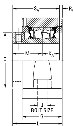
QA Single-Collar Unit
