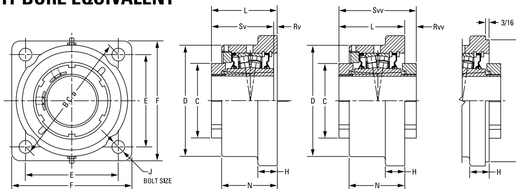
QV Single-Nut Unit (1)
